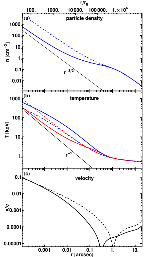
Figure 7. Comparison of the dynamical quantities in the best-fitting solutions with and without conduction: density (top panel), temperature (middle panel), and radial velocity (bottom panel). We show the quantities in the conductive solution (thick solid lines), the quantities in the advective solution (thin lines), and the simple power-laws (thin lines). Shown in the middle panel are the electron temperature T_e (blue/upper solid line) and the ion temperature T_i (red/lower solid line) for the solution with conduction, the electron temperature T_e (blue/lower dashed line) and the ion temperature (red/upper dashed line) T_i for the advective solution. Note that T_e > T_i in the conductive solution, while T_e < T_i in the advective solution. The density is shallower in the flow with conduction. Both density profiles asymptote to n \propto r^{-3/2} and both ion temperature profiles asymptote to T_i \propto r^{-1} in the inner flow. The conductive solution has the sonic point closer in, while the inner asymptotic velocities are comparable in two models.
